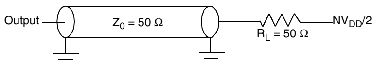
Figure 47. Timers AC Test Load
